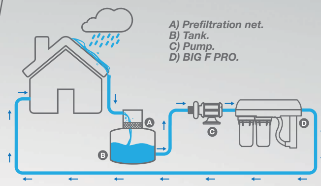
RAINWATER TREATMENT
